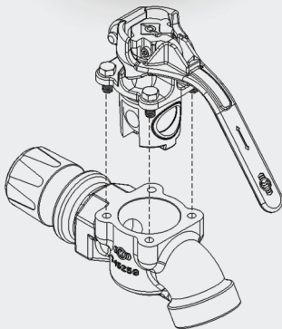
Cartridge based Angle Cock (CBAC) – hex screws torqued to 18-26 ft-lbs.
