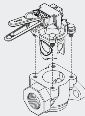
Cartridge Based End Cock (CBEC) – hex screws torqued to 20 – 24 ft-lbs.
