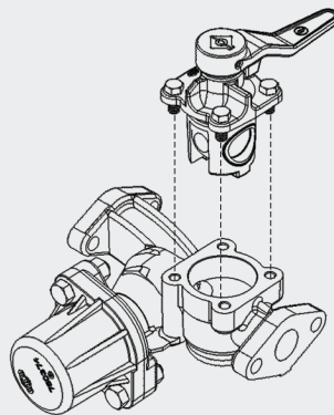
Cartridge Based Dirt Collector (CBDC) – hex screws torqued to 18-26 ft-lbs.
